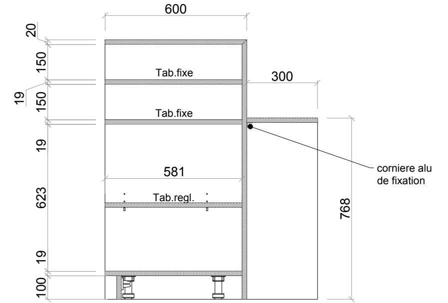
SECTION VIEW HH
